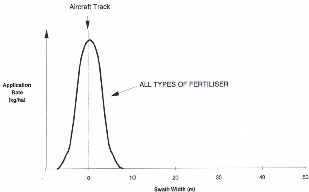
Figure D1 Typical swath pattern under calm conditions – all fertilisers
